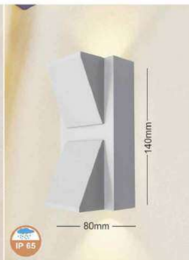
VC 1272 Ø80 H140 Led 5w x 2 > 4000K 410.000đ
